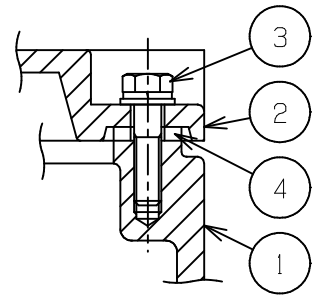
“A”部詳細図(1/4)
