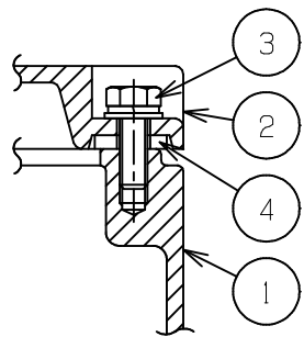
“A”部詳細(1/3)
